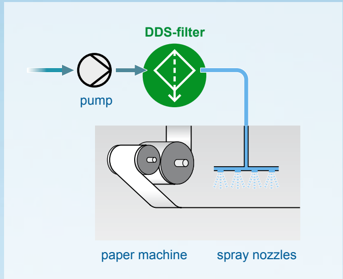
filter for spray water
