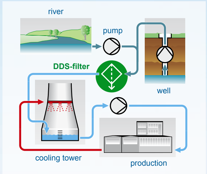
filtration of additional water
