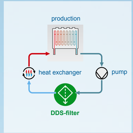
ethylen-glycol refrigeration circuit
