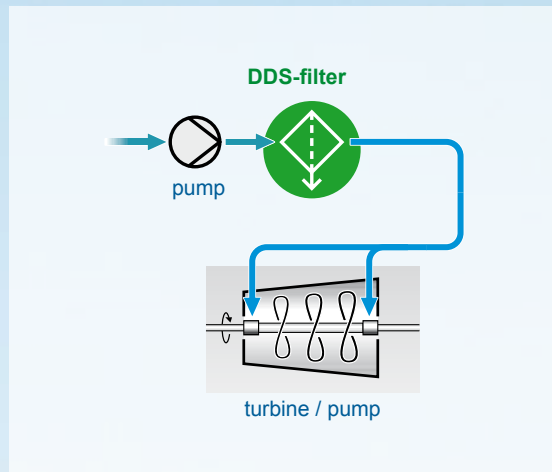
filtration of sealing water
