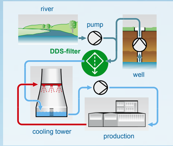
filtration of additional water
