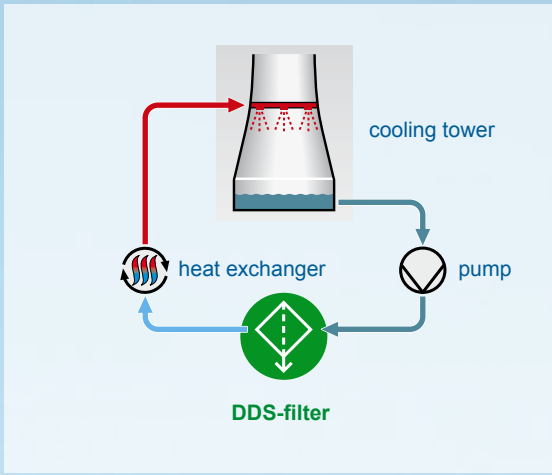
protection of heat exchanger
