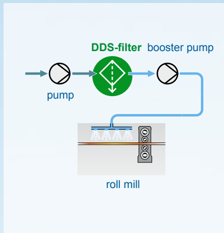
protection of booster pump
