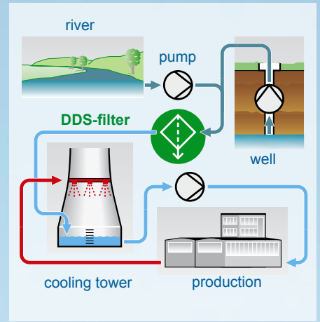
filtration of additional water
